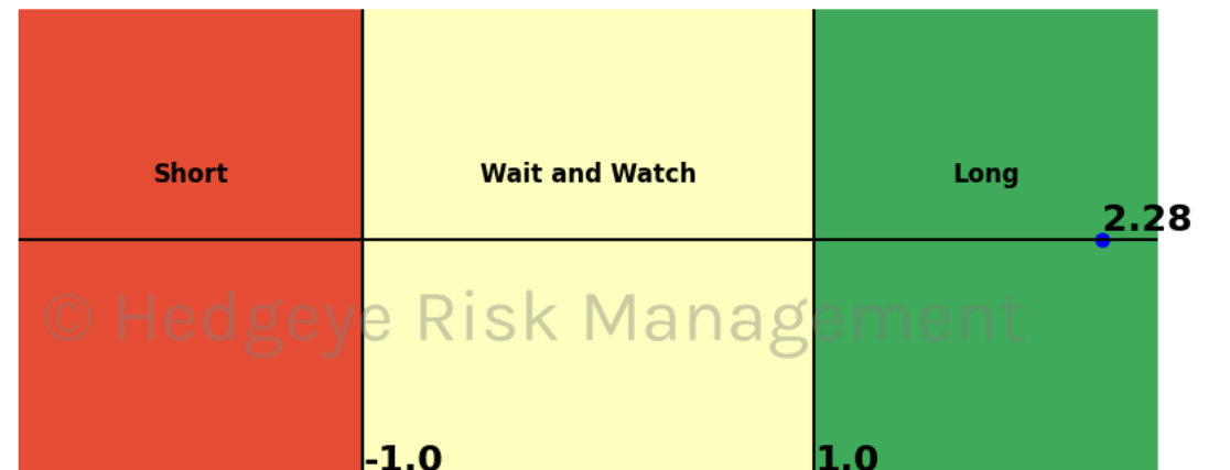
Steel 15 Trading Day Predictions Thresholds of 1.0 and -1.0
