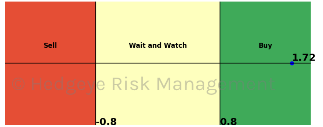
British Pound To US Dollar Cross 15 Trading Day Predictions Thresholds of 0.8 and -0.8
