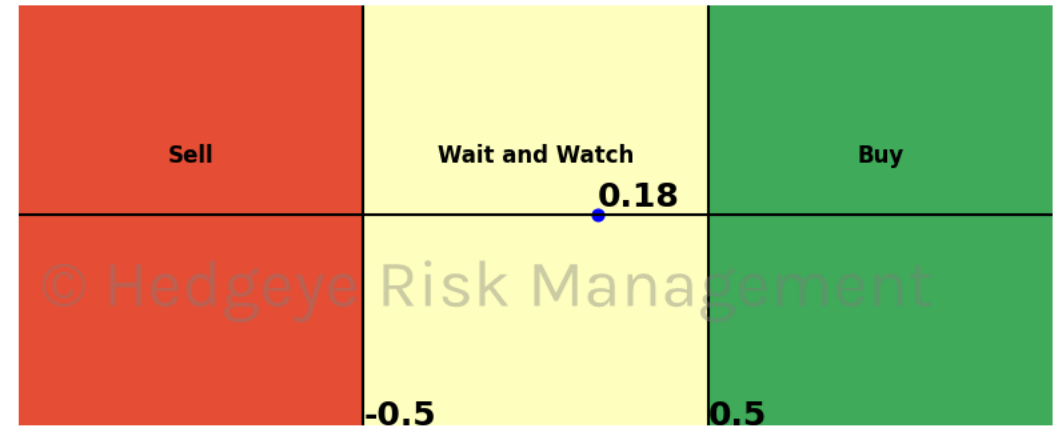
Corn 15 Trading Day Predictions Thresholds of 0.5 and -0.5
