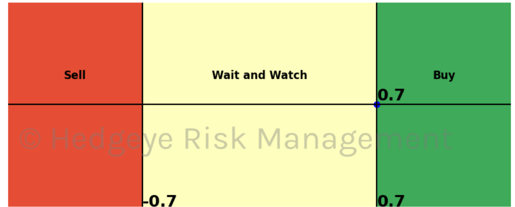
Copper 15 Trading Day Predictions Thresholds of 0.7 and -0.7
