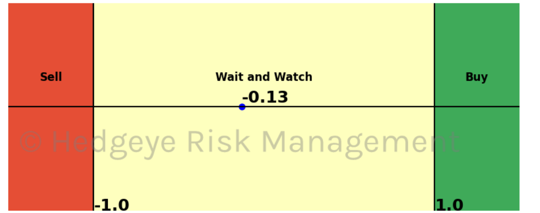
US Dollar To Yen Cross 15 Trading Day Predictions Thresholds of 1.0 and -1.0
