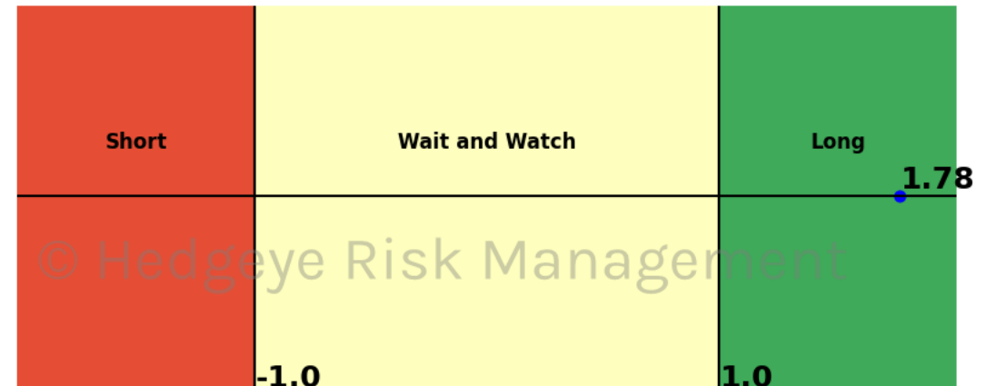
Steel 15 Trading Day Predictions Thresholds of 1.0 and -1.0
